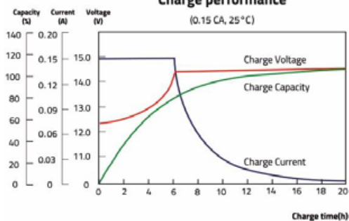
Charge performance
