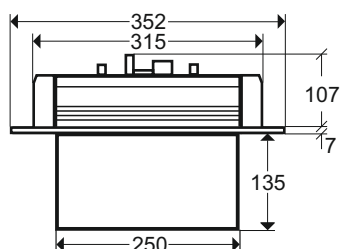
Deckeneinbaumontage (SE):
