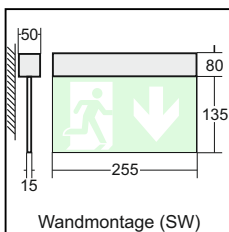
Wandmontage (SW)
