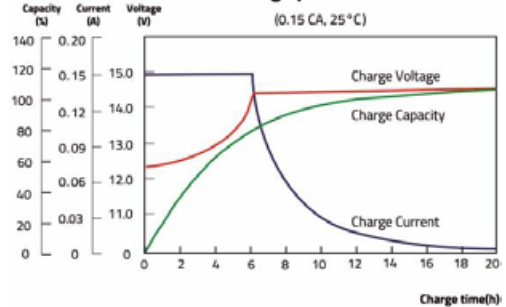
Charge performance
