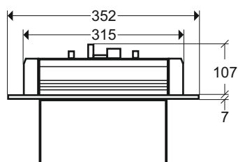
Deckeneinbaumontage (SE):
