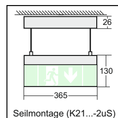
Seilmontage (K21...-2uS)
