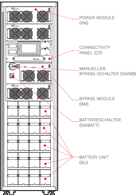
MPW 130 CBC MPW Combo Cabinet 42–126 kW (Vorderseite)
