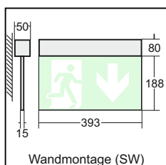
Wandmontage (SW)
