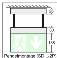
Pendelmontage (SD...-2P)
